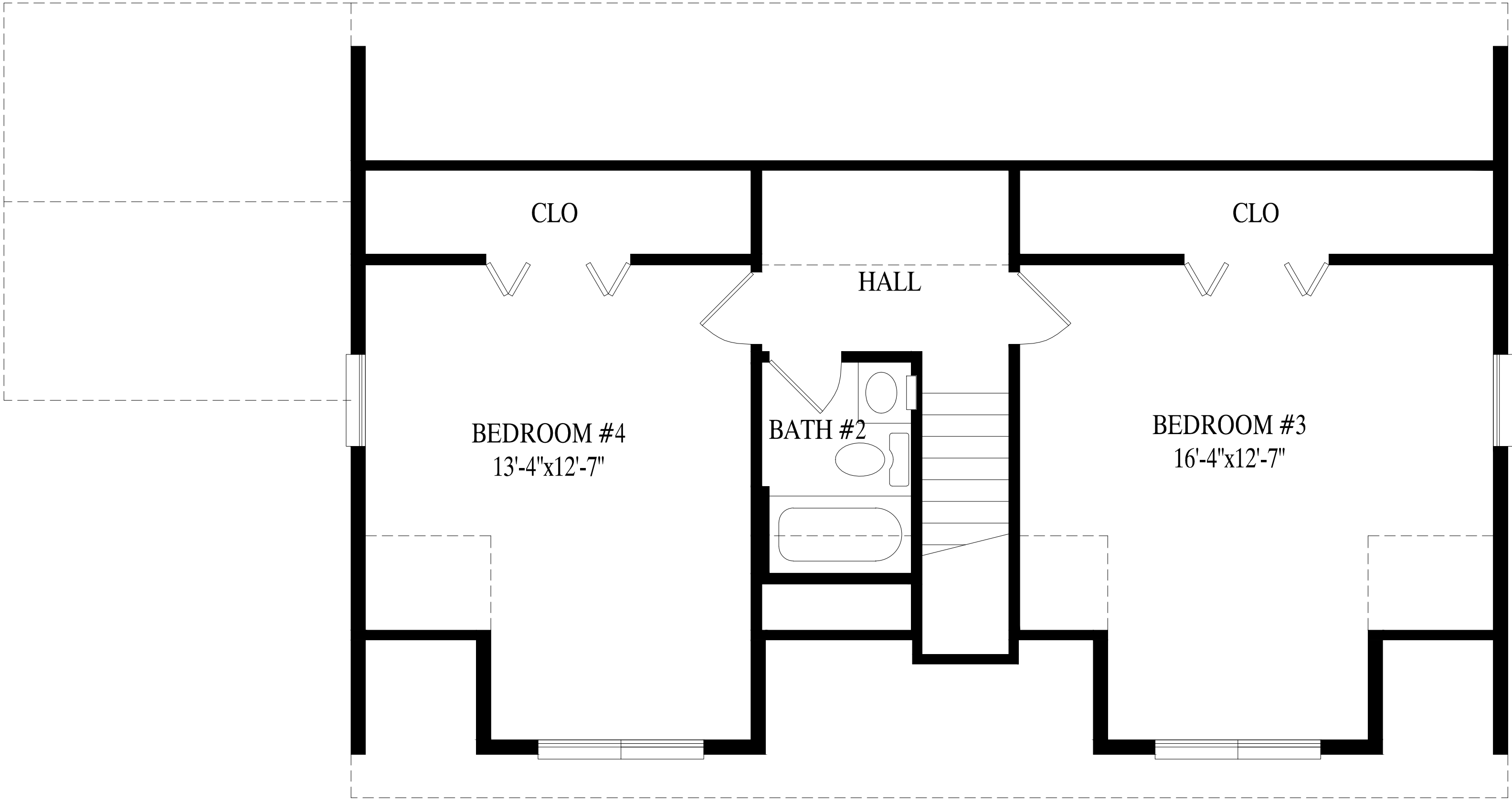
Proposed 2nd Floor - 745 sq. ft.
